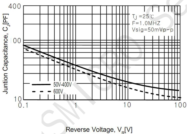
Figure 3. Junction Capacitance
